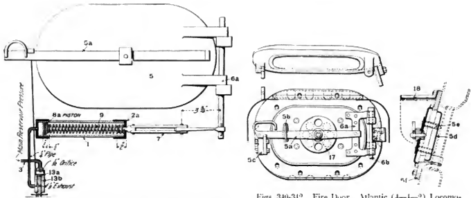
Fig. 339. Brewer's Pneumatic Fire Door Opener.
